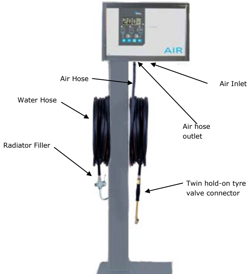
D25 Air and Water Hoses
